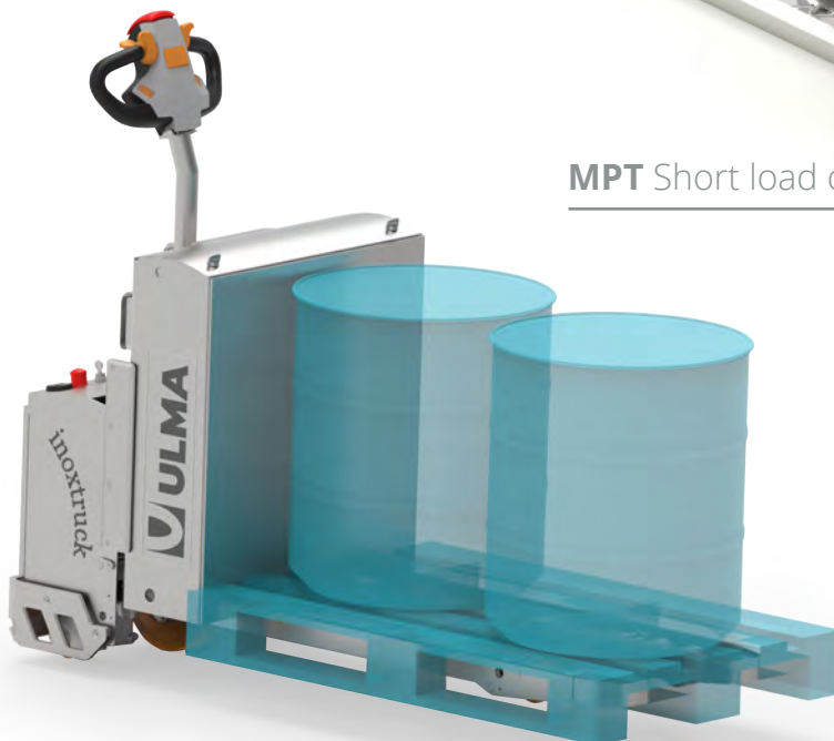
EPT Electronic pallet truck
