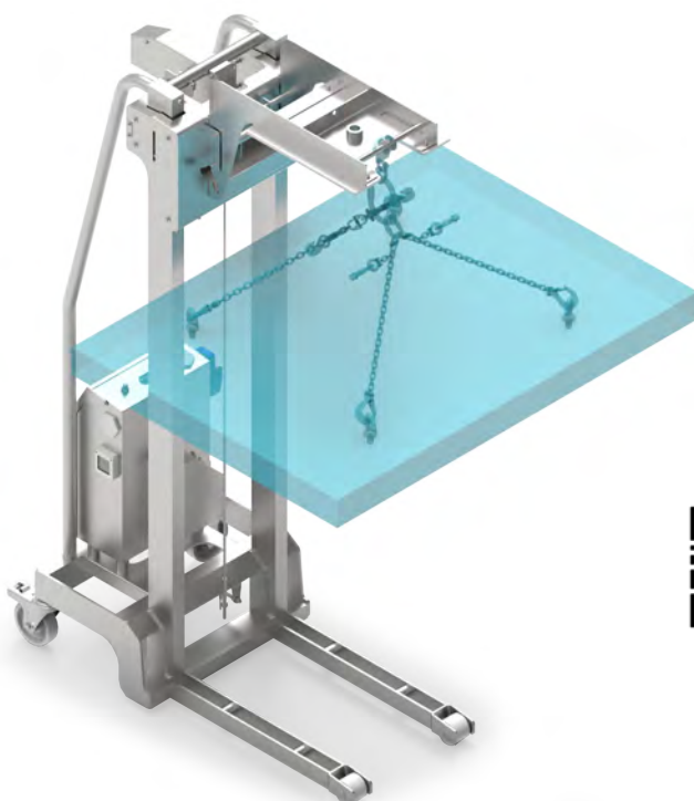
EMS for mould handling
