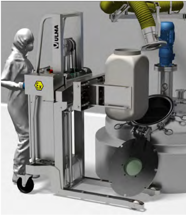
EMS Drum Rotator Lifter Ex-Proof
