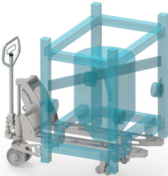
MPT special 300 mm fork height
